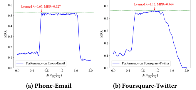
Figure 5: MRR with different \lambda . Our learned \lambda consistently achieves the best MRR on both datasets.
